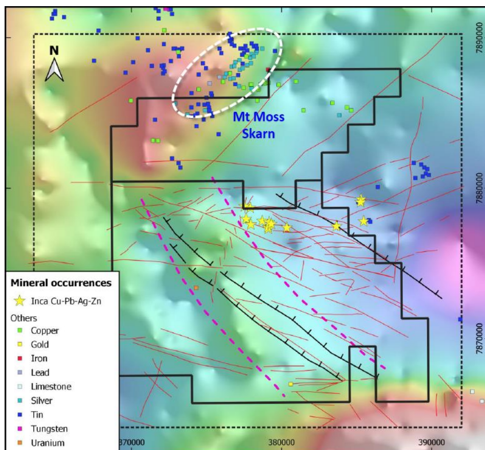
Figure 3: Gridded regional gravity image over MaCauley Creek. While regional data is of coarse resolution, two sub-parallel gravity gradients (pink dashed lines) traverse the Project and may have allowed intrusion of granitic and porphyry stocks. The eastern gravity gradient lies proximal to the cluster of mineral occurrences (yellow stars) in the central porphyry target area.
