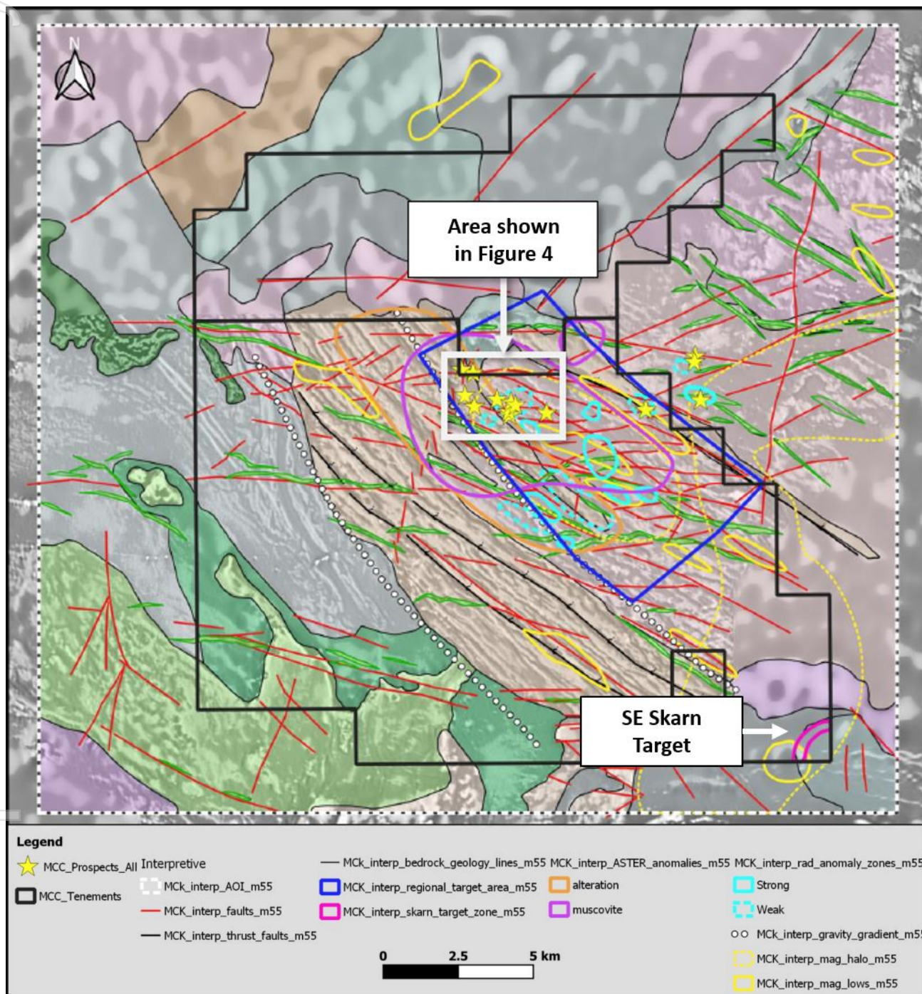
Figure 1: Independently-generated magnetic TMIRTP-1VDAGC greyscale image of the MaCauley Creek Project area with digitised interpretation linework added as per legend. The large new porphyry target is shown as a large dark blue rectangle. Within this area, note the coincidence of strong radiometric potassium anomalies (light blue lines), deep magnetic lows (yellow lines), alteration halos (purple and orange lines). The old mine workings and mineralised prospect areas (yellow stars) occur within this multi-layered target area.
