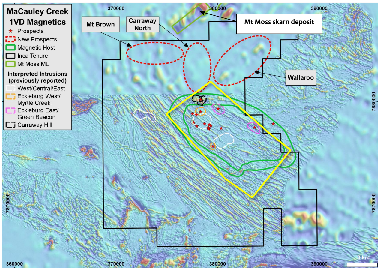
Figure 2: A 1VD (vertical derivative) magnetics image showing the previously identified Mt Brown, Carraway North and Wallaroo epithermal-porphyry-skarn targets. The NEW porphyry target is also shown (solid yellow line)
